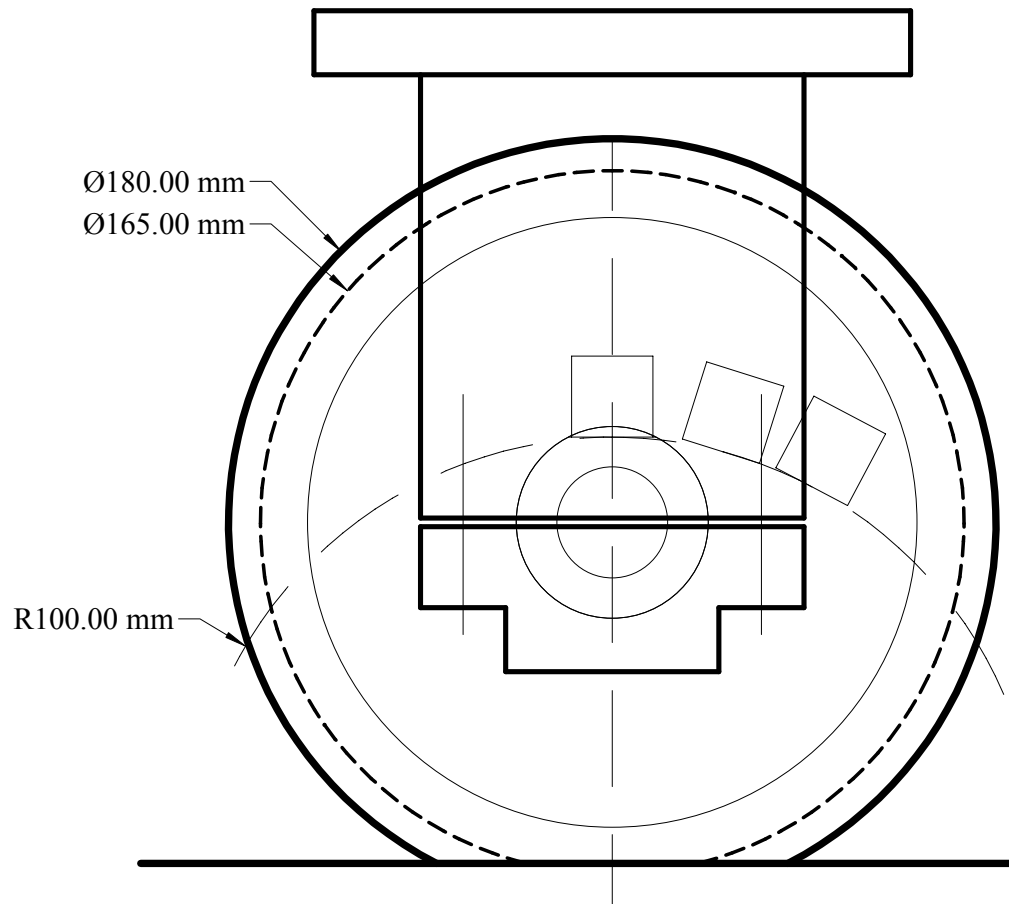
PL180 wheel probe outlines
